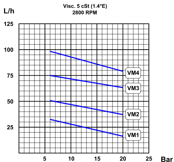
Nozzle capacity
